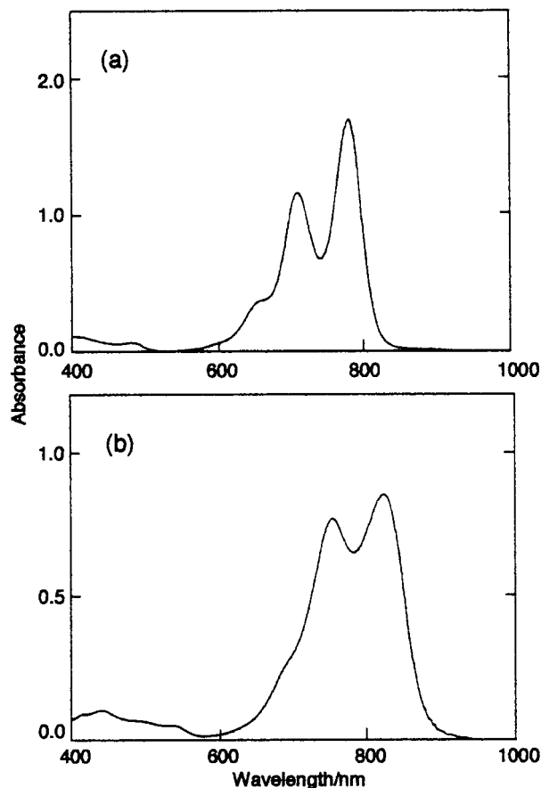
Fig. 2 The UV-vis absorption spectra of (a) 11 and (b) 12 in \text{CHCl}_3 at 20\text{ }^\circ\text{C} . The concentrations are 1.7 \times 10^{-5} and 9.4 \times 10^{-6} M, respectively.
